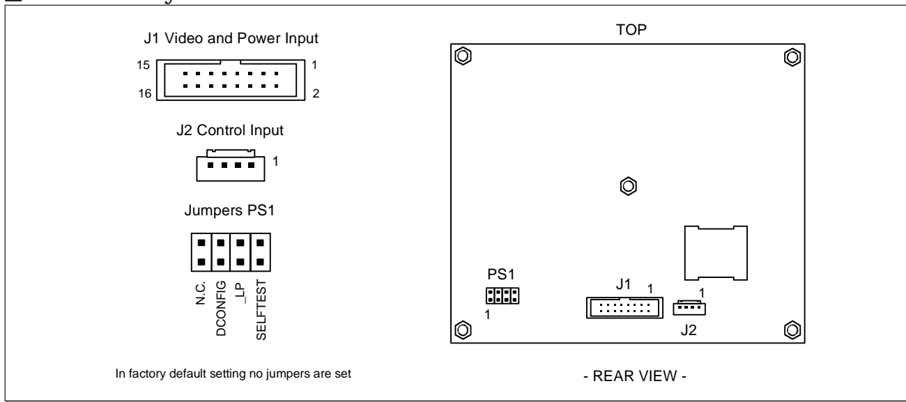
Fig 1. The input connectors and programmable jumpers on EL320.256-F6 and -FD6 displays.
