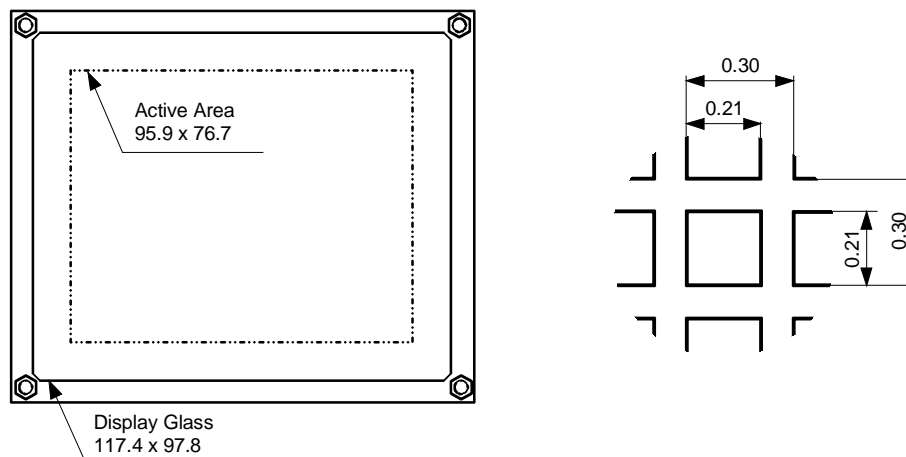
Fig 2. EL320.256-F6 and -FD6 display viewing area characteristics.
