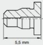
Throttle for FF 4-2 up to 32
