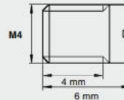
Throttle screw for FF 4-12/30/60/120/250
