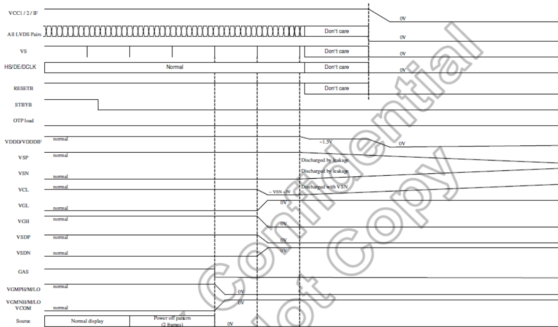
Figure 6.3: Power-off sequence with PFM
