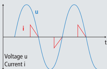
Leading edge phase control
