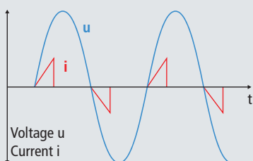
Trailing edge phase control
