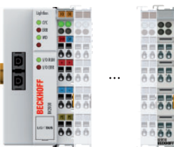
Operation with up to 64 Bus Terminals to one Bus Coupler with KL9010 bus end terminal
